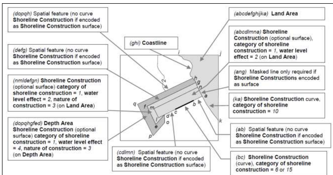
Figure 8-1 – Shoreline constructions
