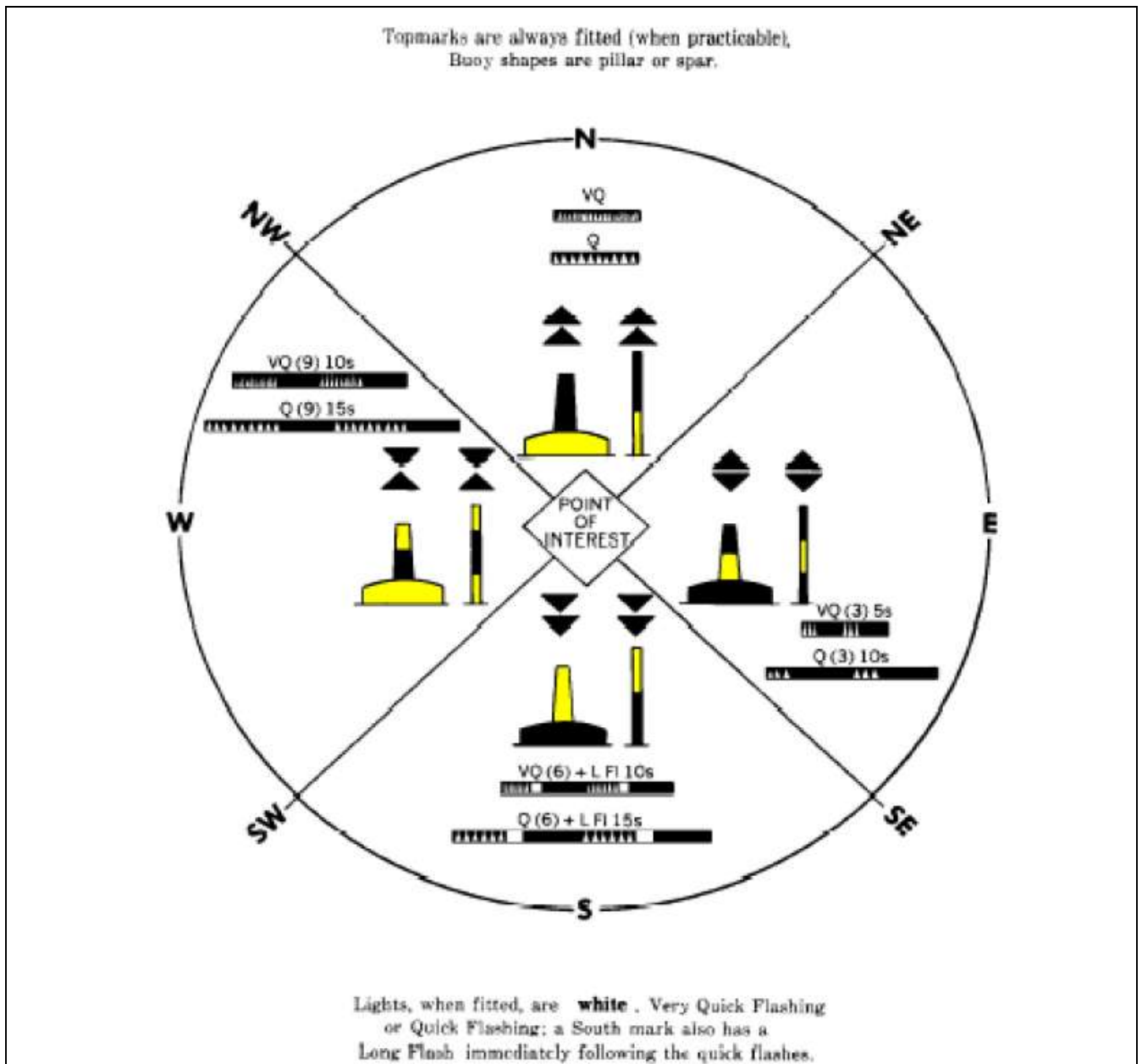
Figure 20-2 – IALA cardinal buoys – Characteristics
