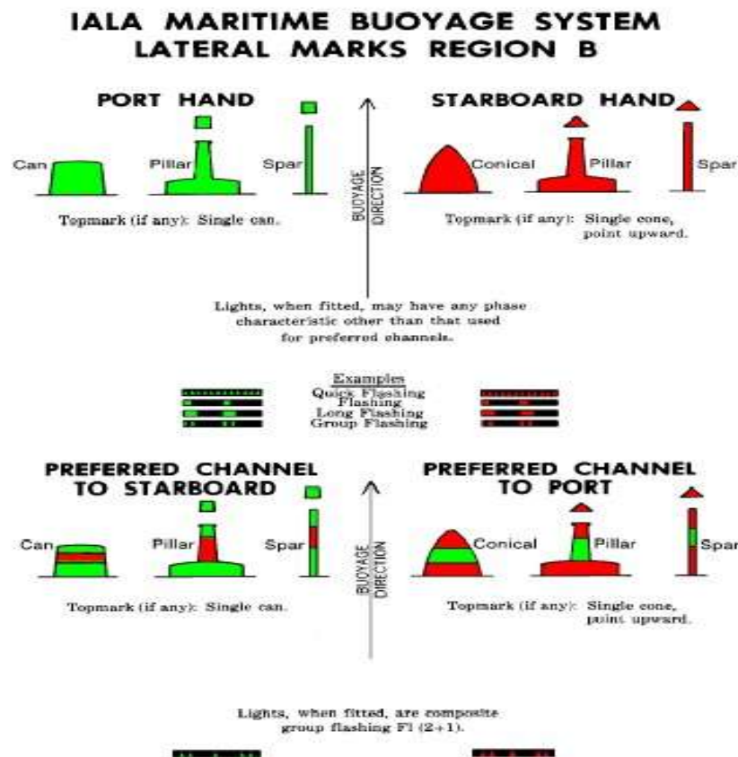
Figure 20-1 – IALA lateral buoys – Characteristics
