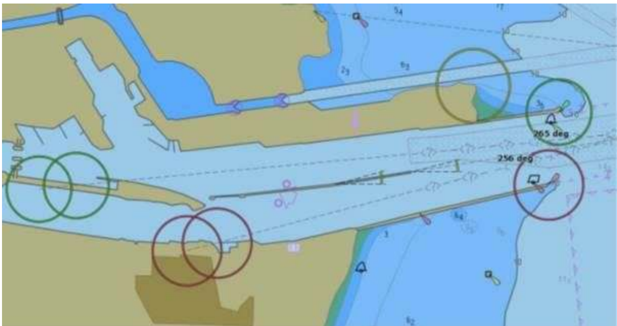
Figure 19-1 – Omnidirectional light display in Inland ECDIS or ECS
