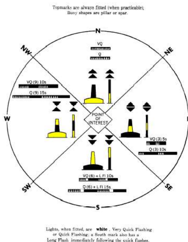
Figure 20-6 – IALA cardinal beacons – Characteristics
