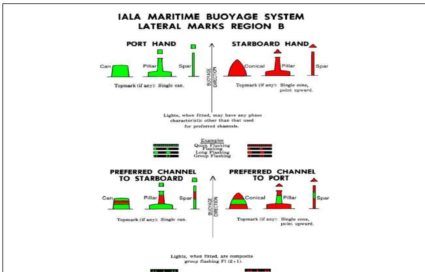
Figure 20-5 – IALA lateral beacons – Characteristics
