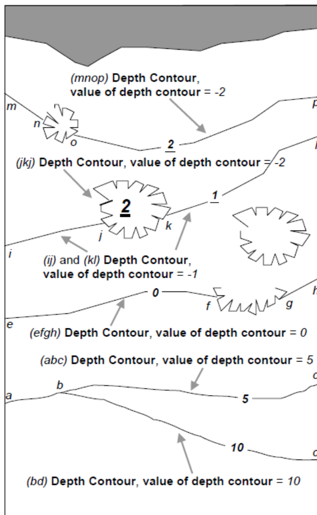
Figure 11-2 – Depth contours
