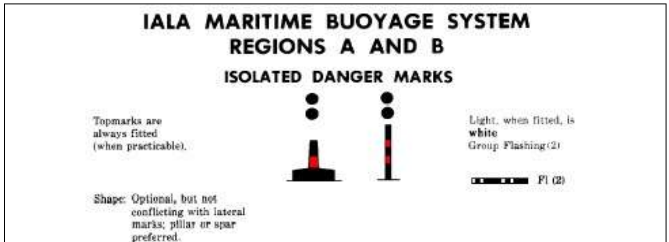
Figure 20-7 – IALA isolated danger beacons – Characteristics
