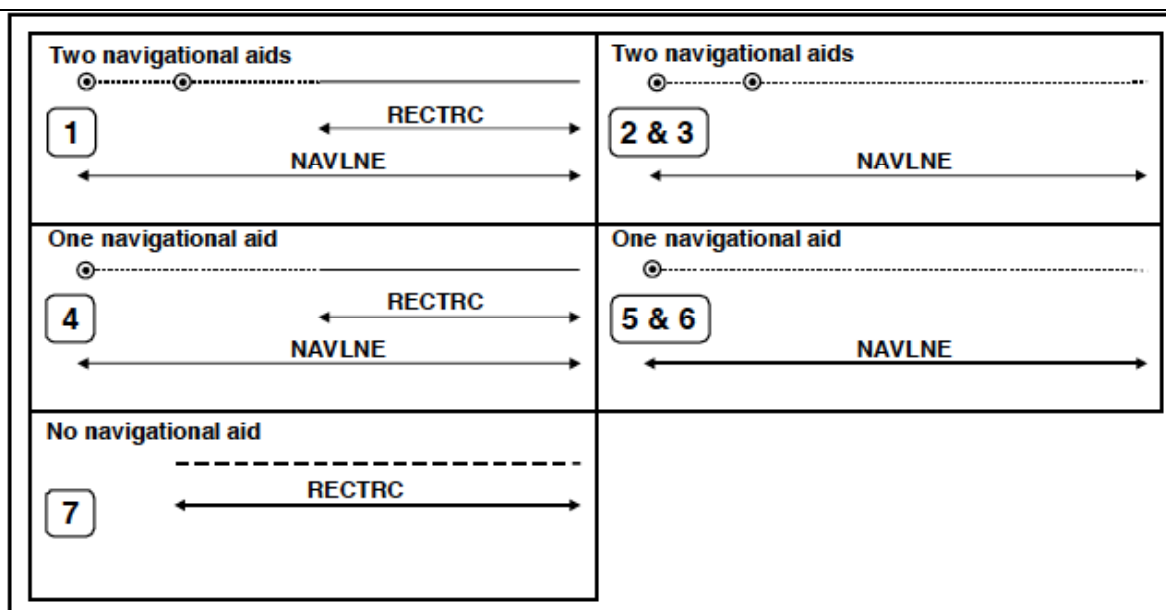
Figure 15-5 – Navigation lines – Geometry encoding
