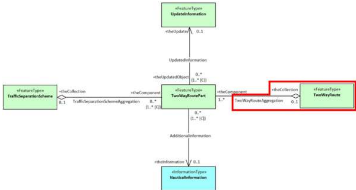
Figure 25-1 – Two-Way Route Part UML relationship diagram
