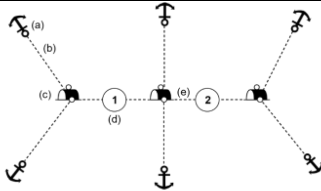
Figure 8-2 – Mooring trot
