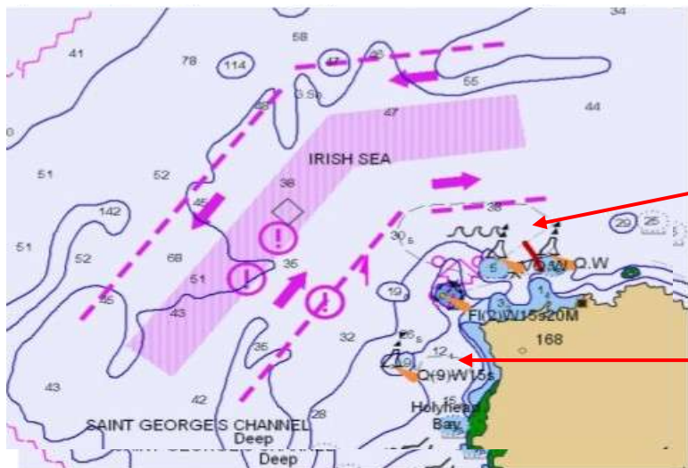
Figure 2-9 – Traffic Separation Scheme with appropriate masking
