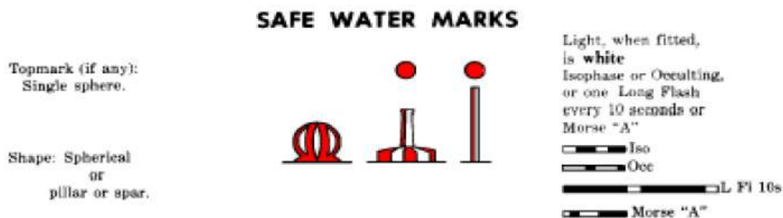
Figure 20-4 – IALA safe water buoys – Characteristics
