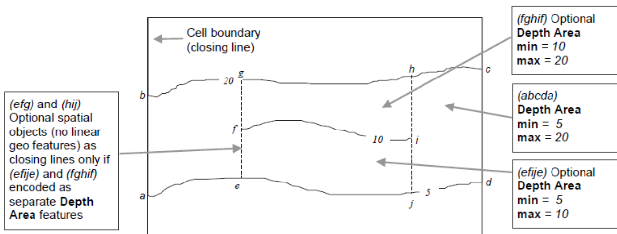
Figure 11-3 – Geometry of depth areas
